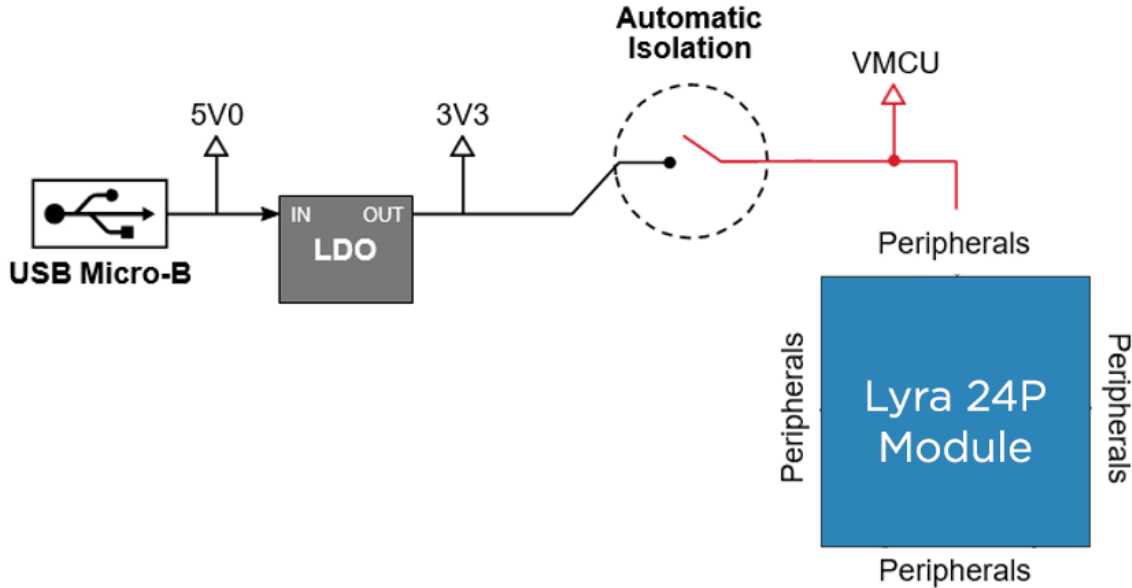
Figure 3: Lyra 24P DVK power diagram
