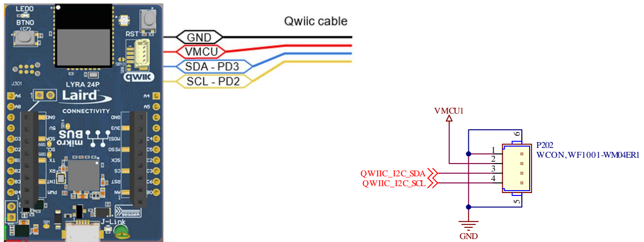
Figure 10: Qwiic connector
